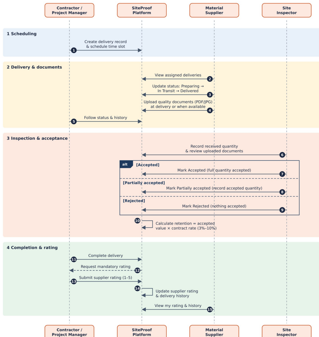
Figure 2. Business sequence diagram of the Material Delivery Closed-Loop.
